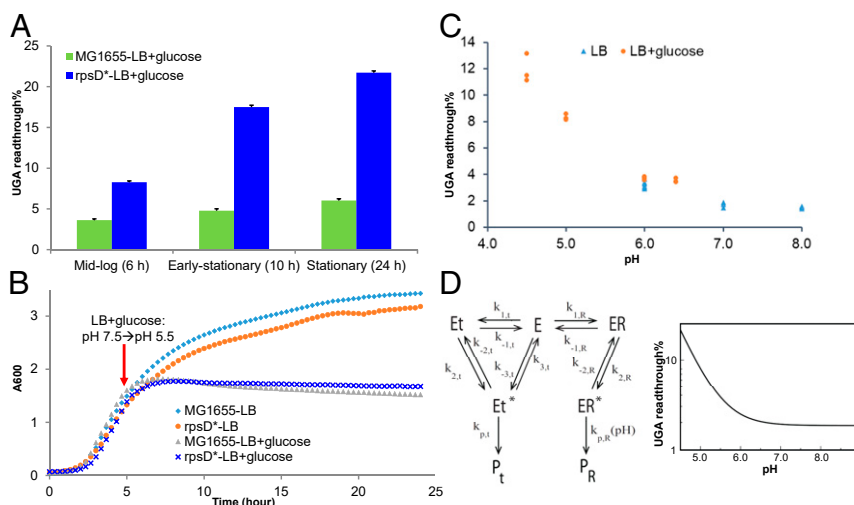
Fig. 2. Excess carbon increases UGA readthrough by lowering pH. (A) E. coli cells carrying the mCherry-TGA-YFP reporter were grown in LB or LB with 1% glucose. At 6, 10, and 24 h, fluorescence was determined using a plate reader, and the UGA readthrough levels were calculated. Error bars represent one SD ( n \geq 3 ). (B) Growth curve of E. coli in LB or LB with 1% glucose. A pH shift from 7.5 to 5.5 was observed at 5 h in the LB glucose media. Excess glucose caused growth arrest at 7 h, correlating with a substantial increase in the UGA readthrough level. (C) E. coli MG1655 was grown in buffered LB or LB glucose for 24 h, and the UGA readthrough level was determined as in A. The pH of the media was determined at 24 h. (D) Mathematical modeling of the pH effect on UGA readthrough. R stands for release factor (RF2); the near-cognate aminoacyl-tRNA (t) is the wrong substrate that suppresses UGA; P_R is the hydrolyzed peptide, and P_t represents the elongated peptide. Modeling results suggest that when pH drops to below 6, the UGA readthrough error substantially increases. The kinetic parameters used for modeling are from references (33, 34). See SI Appendix for details of modeling.
